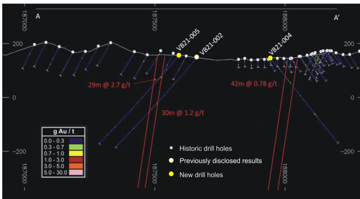
Figure 2 – Section 8436400N View of VB21-004 and VB21-005 with VB21-002 Assay Results
