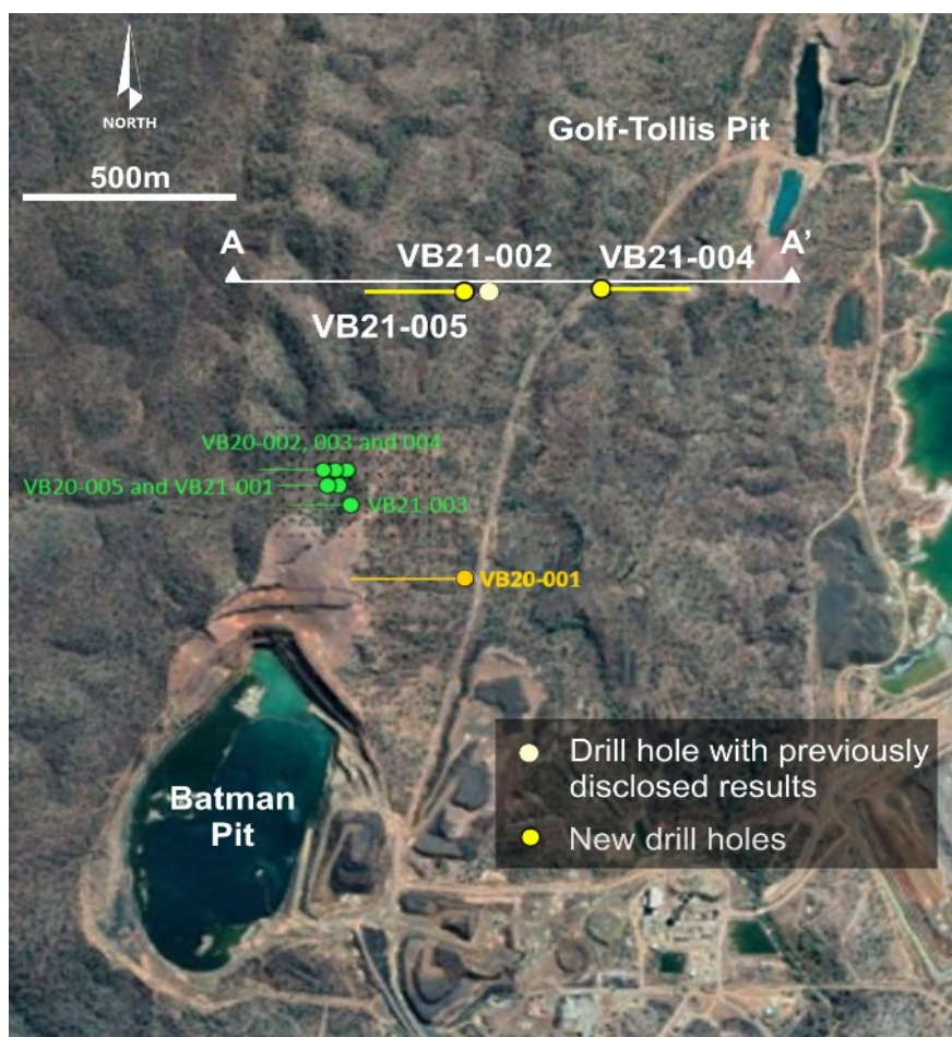
Figure 1 – Plan View of Drill Holes and Cross Section Locations
