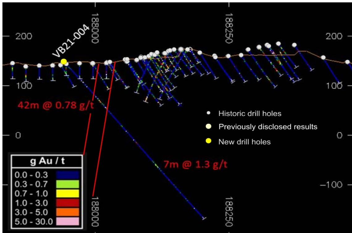
Figure 4 – Section 8436400N Enlarged View of VB21-004 and Historic Drilling
