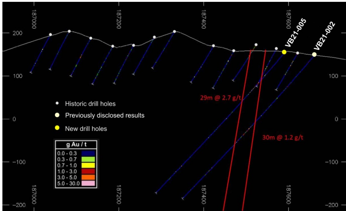
Figure 3 – Section 8436400N Enlarged View of VB21-005 and VB21-002 Drilling Assay Results
